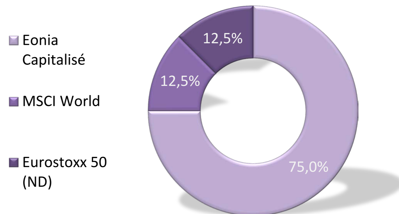
Composition Benchmark
