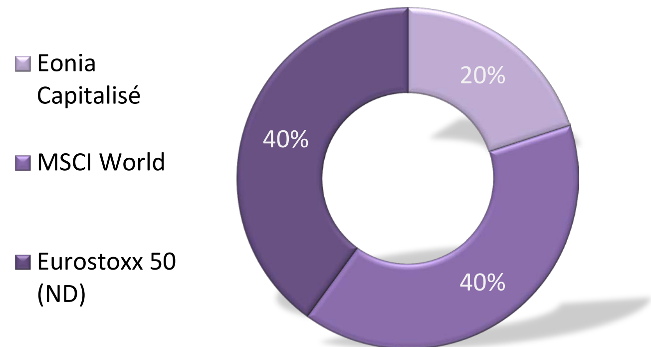
Composition Benchmark
